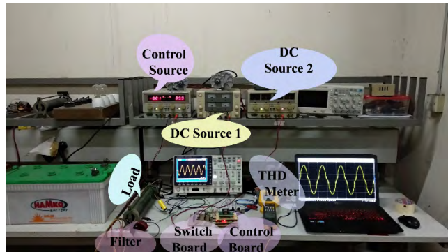
FIGURE 31. Complete hardware setup for the proposed modified 5-level CHB inverter.
