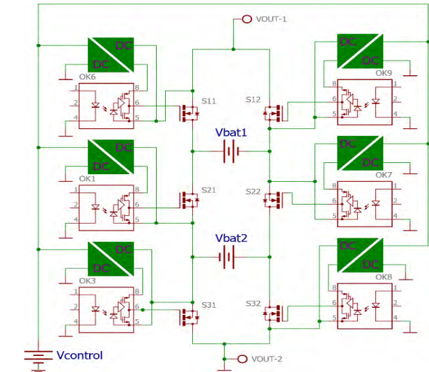
FIGURE 30. Proposed inverter with MOSFET control mechanism. Isolated DC-DC converter modules are needed for each MOSFET gate driving mechanism, which are powered up by totem-pole drive optocouplers, and they receive signals from the microcontroller.
