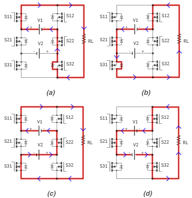
FIGURE 4. Generation of four distinct voltage levels in the modified 5-level cascaded H-bridge multilevel inverter, when operated by switching sequences shown in Table 1. (a) +V . (b) -V . (c) +2V . (d) -2V .
